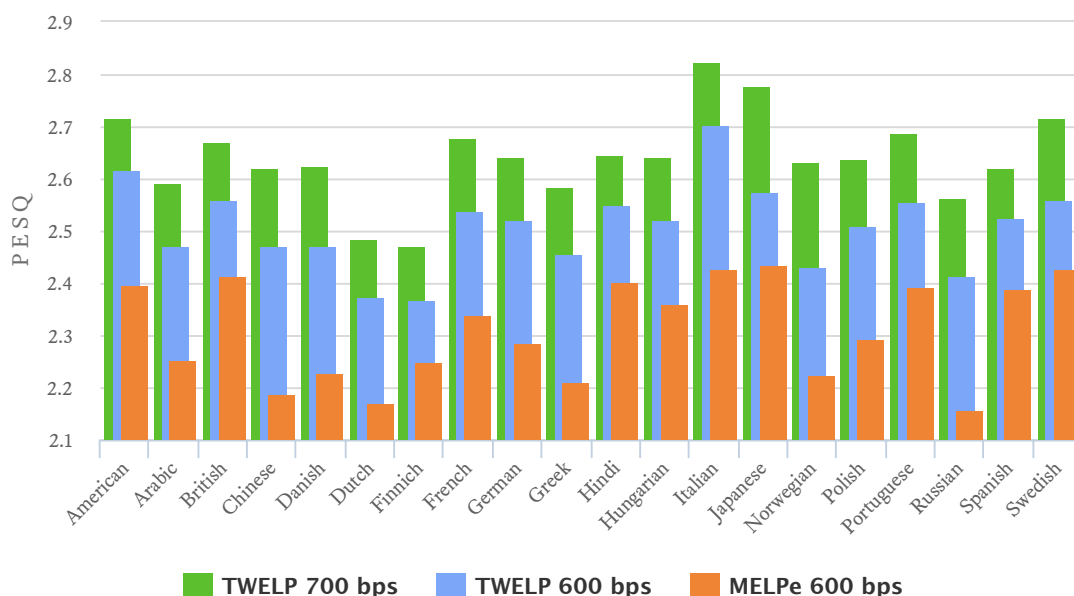
TWELP 700 bps vs TWELP 600 bps and MELPe 600 bps
